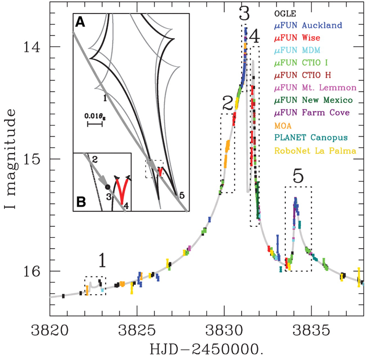
Fig. 5.— OGLE-2006-BLG-109
